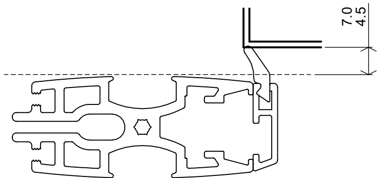
Q-Lon foam seal - QL7066
