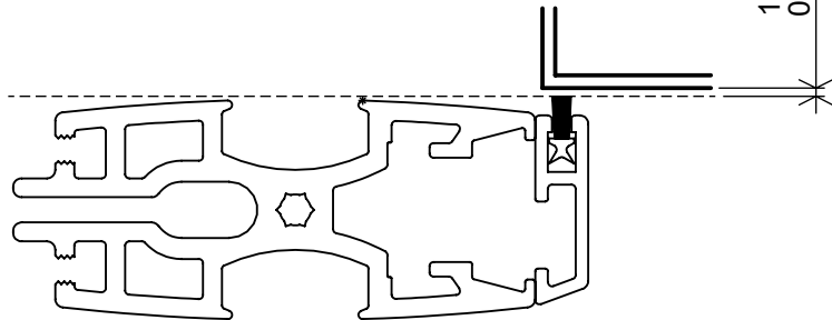
8mm Brush seal SEL-043
